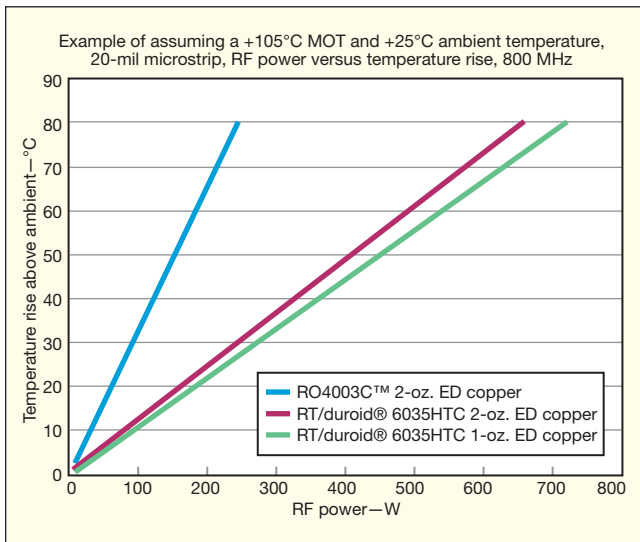
4. This plot compares the power-handling capabilities of RO4003C, RT/duroid 6035HTC with 2-oz.copper, and RT/duroid 6035HTC with 1-oz.copper at 800 MHz.
