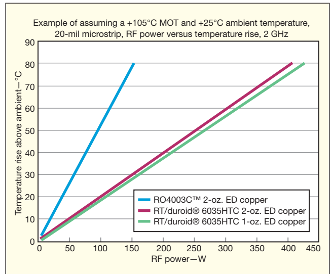
5. This plot compares the power-handling capabilities of RO4003C, RT/duroid 6035HTC with 2-oz.copper, and RT/duroid 6035HTC with 1-oz.copper at 2 GHz.
